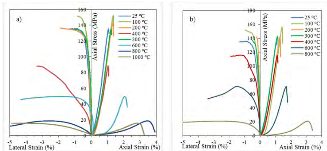
Figure 7. Stress-strain curves during loading for heat-treated specimens (a) for rapidly cooled specimens (b) for slowly cooled specimens.
