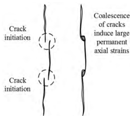
Figure 14. Conceptual model for crack coalescence results for permanent axial strains and crack damage. Modified after Eberhardt [49].
